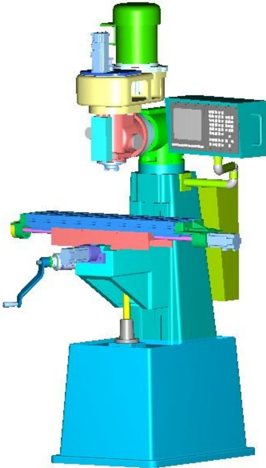
NC milling machine 數控銑床 CF-A2NC
