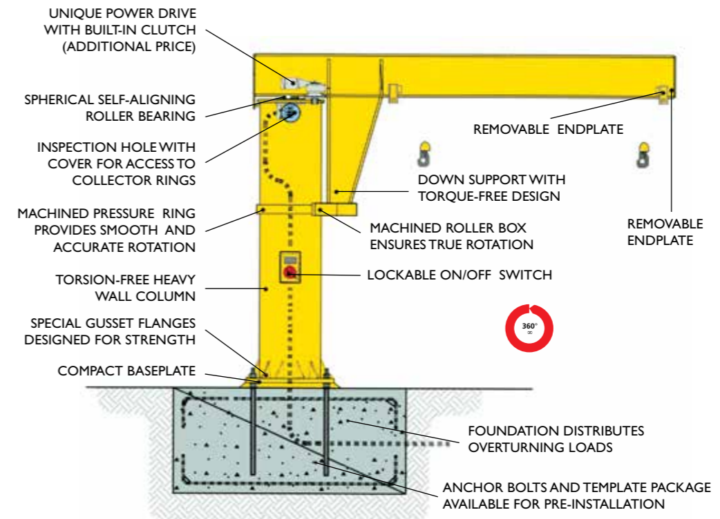
Type KBK slewing jib cranes, wall- and column-mounted
