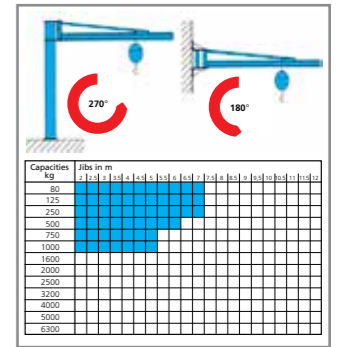
Type KBK slewing jib cranes, wall- and column-mounted
