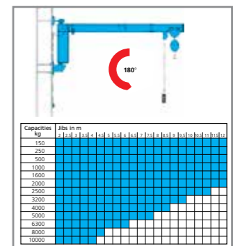
Type G Wall mounted slewing jib cranes
