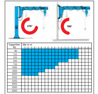
Type AS/AW slewing jib cranes, wall- and column-mounted
