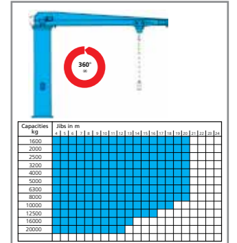
Type B slewing jib cranes
