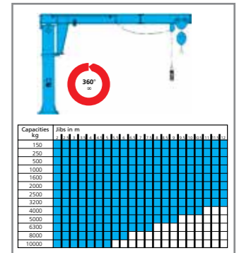
Type M slewing jib cranes
