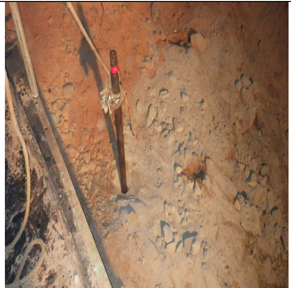
將 ATD 鋼管置入孔中 啓動 Place ATD Tube in the hole and blasting
